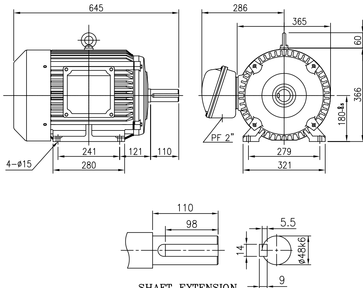
SHAFT EXTENSION
