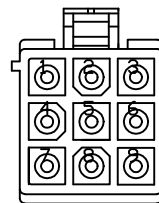
AMP 172169-1 PLUG 9P AMP 170359-1 PIN
