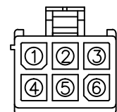
AMP 172168-1 Plug 170360-1 PIN
