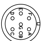
Lead Wire 선번호 PIN 번호 U A V B W C Ground D Brake + E Brake - F
