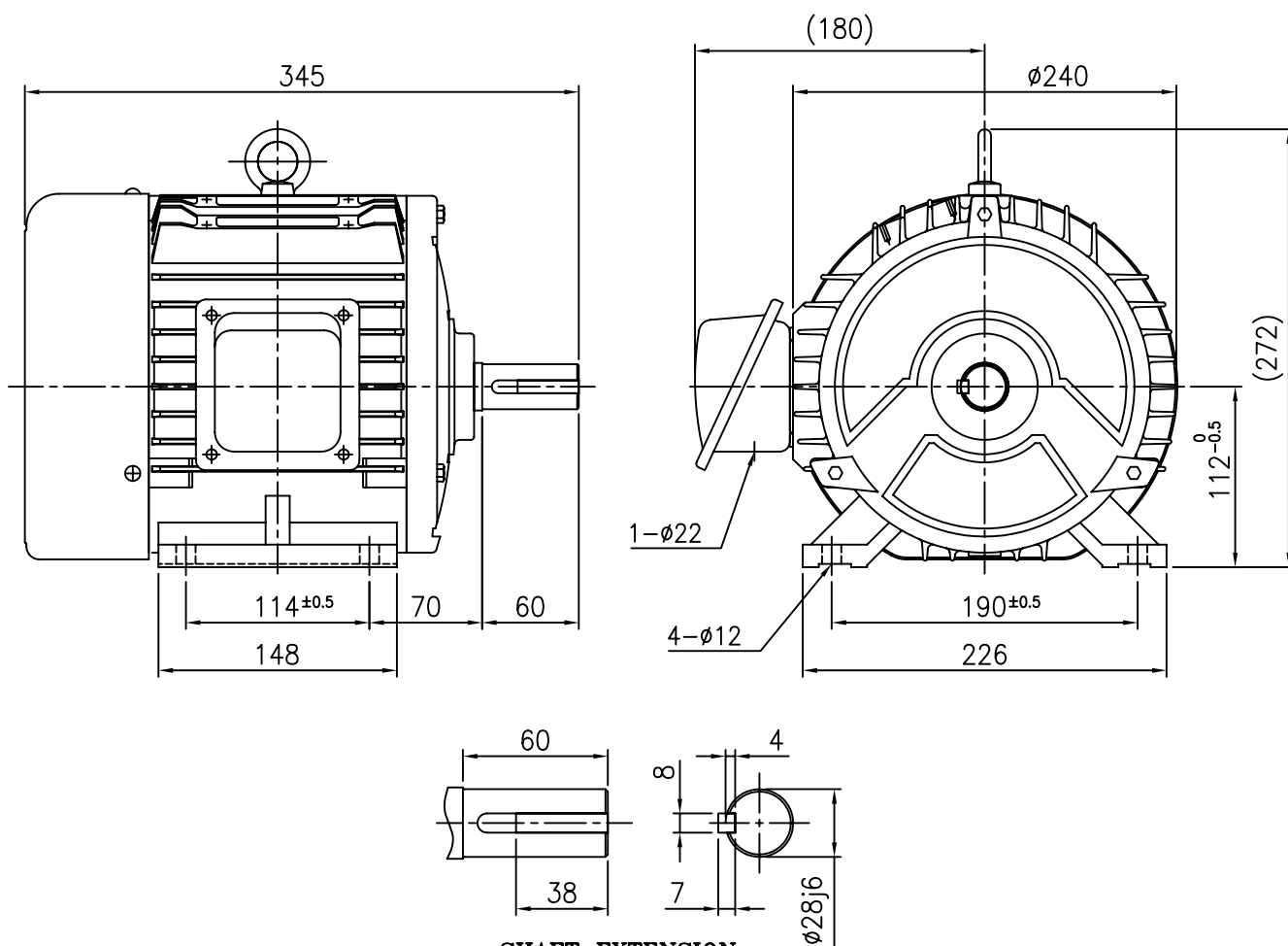
SHAFT EXTENSION
