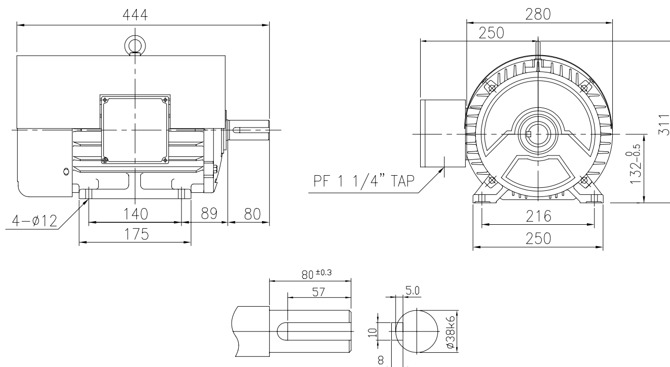
SHAFT EXTENSION
