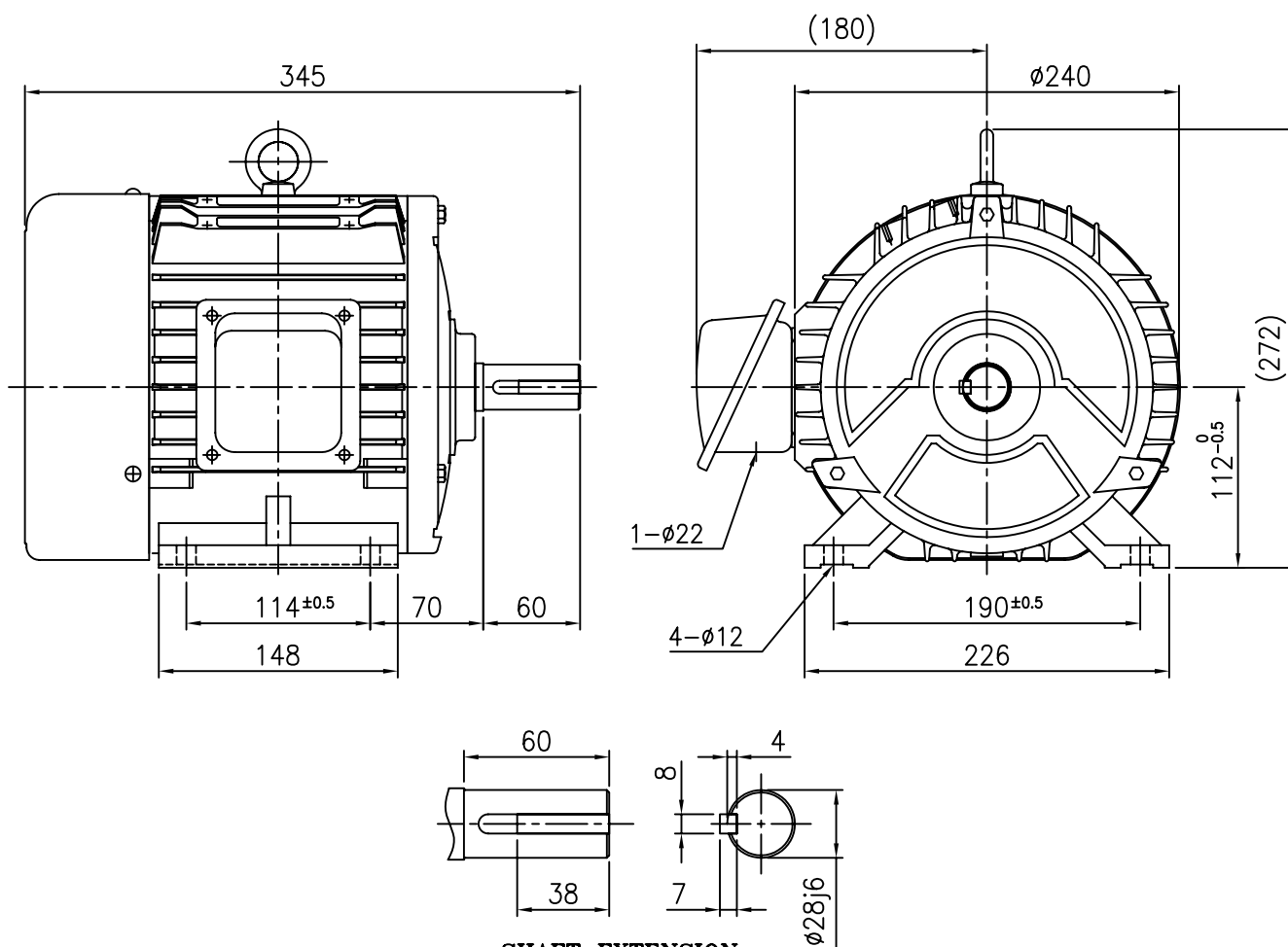
SHAFT EXTENSION
