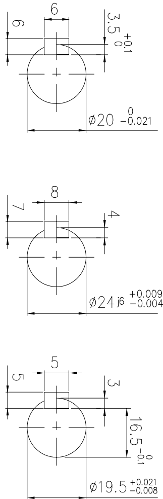
DETAIL "K"
