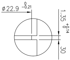
DETAIL "K"
