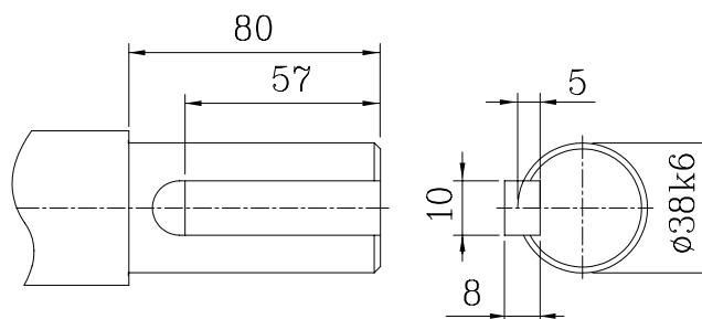
SHAFT EXTENSION
