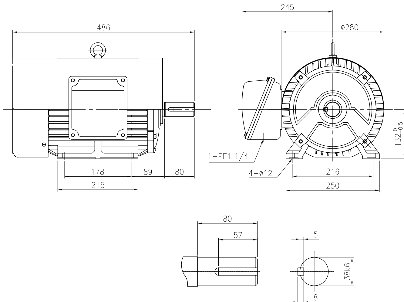
SHAFT EXTENSION
