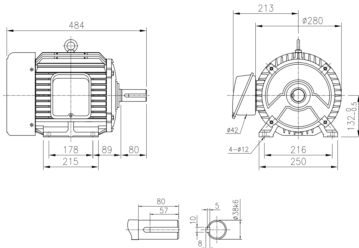
SHAFT EXTENSION
