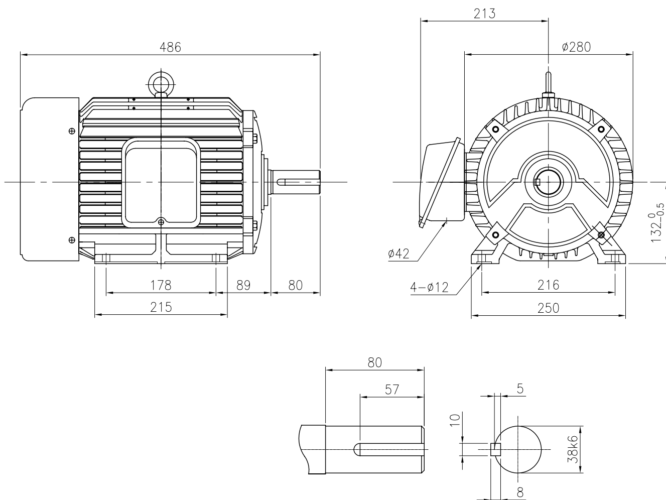
SHAFT EXTENSION
