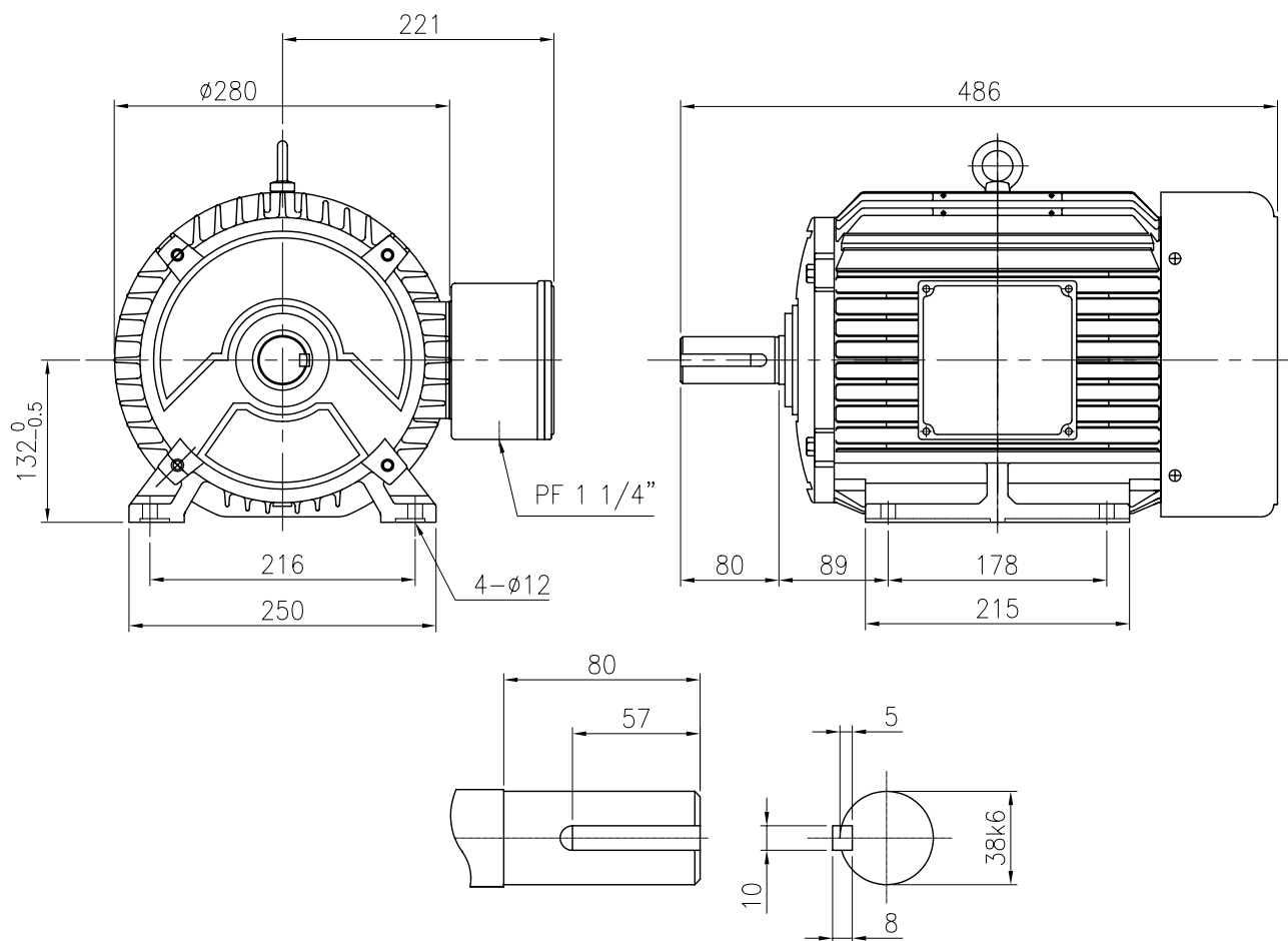
SHAFT EXTENSION
